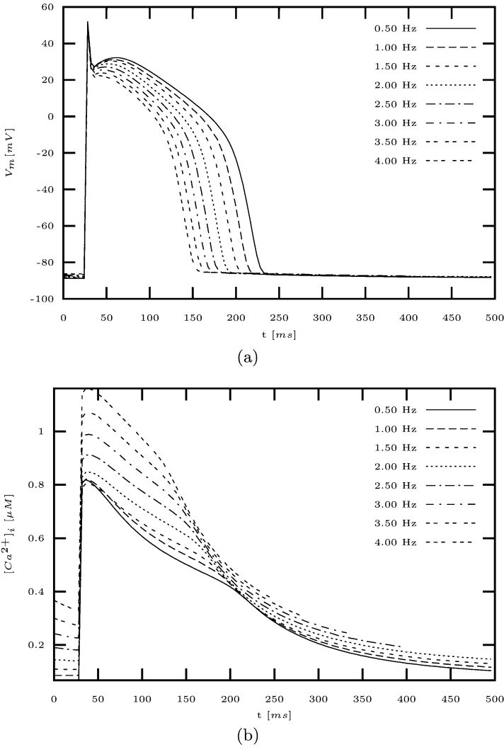
Fig. 7.16. Simulations with an enhanced Luo-Rudy phase-2 model. (a) Transmembrane voltage V_m and (b) intracellular calcium concentration [Ca^{2+}]_i are dependent on the stimulus frequency. For each frequency a single course of the transmembrane voltage and intracellular calcium concentration, respectively, is visualized.
