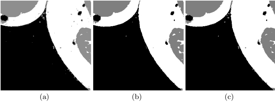
Fig. 5.6. Opening operator applied to grey level image (from [37]). (a) Original image. The image resulting from application of (b) erosion filter and (c) opening operator. The opening operator consists of an erosion followed by a dilation. Small artifacts are erased and the object's area is reduced by the erosion filter. The object's area is preserved by the opening operator.
