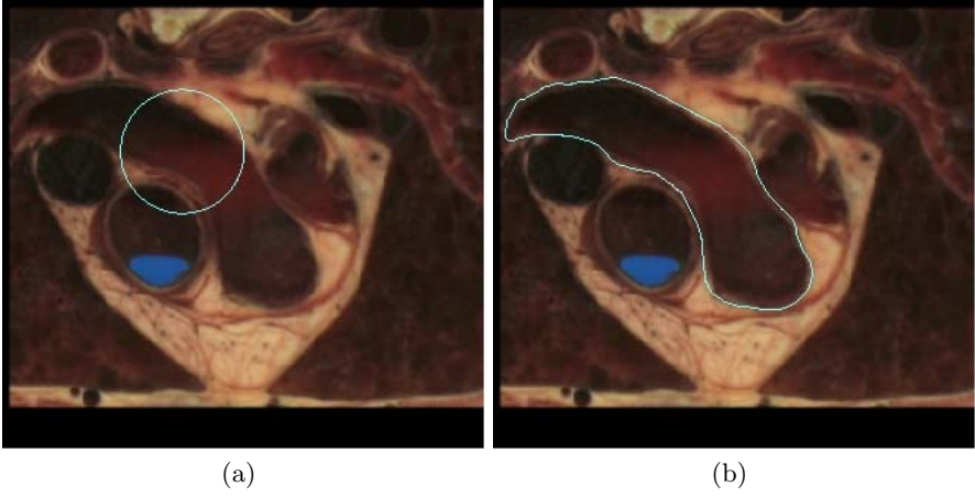
Fig. 5.16. Interactive deformation of triangle mesh for segmentation of aorta. (a) The image overlaid with an initial triangle mesh and (b) manually adapted triangle mesh. The user adapts the mesh by picking and moving of mesh elements. The moving leads to a local deformation with controllable area of influence. The user interaction is performed in two-dimensional slices of selectable orientation and position. The resulting mesh deformation is three-dimensional.
