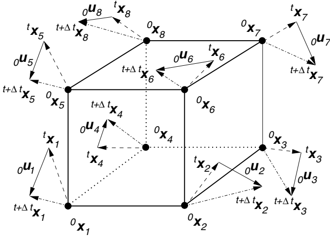
Fig. 4.7. Deformation and incremental displacements in hexahedron. The coordinates of node points {}^0x_i in the Lagrangian configuration are changed to the coordinates {}^tx_i at time t . The incremental displacement {}^0u_i leads to the coordinates {}^{t+\Delta t}x_i at time t + \Delta t .
