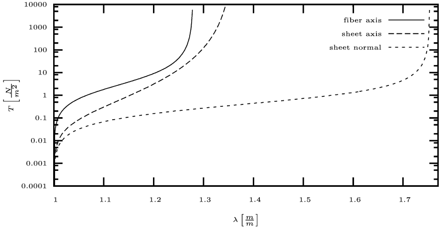
Fig. 8.7. Unidirectional second Piola-Kirchhoff stress \mathbf{T} derived from hyperelastic material law of Hunter-Nash-Sands for epicardial canine myocardium. The stress is shown versus the stretch ratio \lambda and is dependent on three orthogonal axes.
