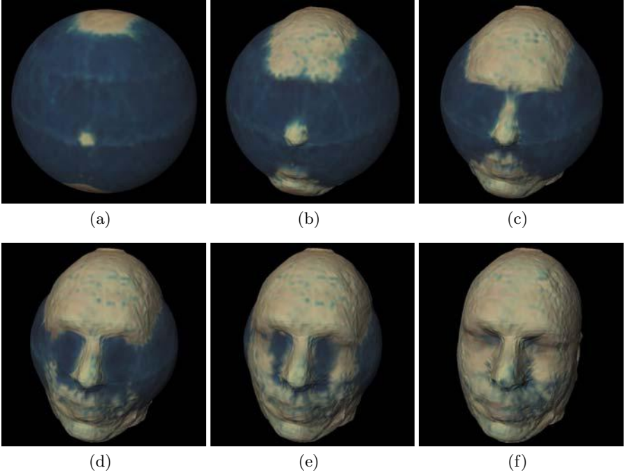
Fig. 5.13. Three-dimensional image segmentation with active contour model (from [37]). (a) The initial contour is a sphere. The resulting advance of the contour is shown in (b)-(f). The energy includes stretch and image energies. The triangle mesh is dyed with colors from the image.
