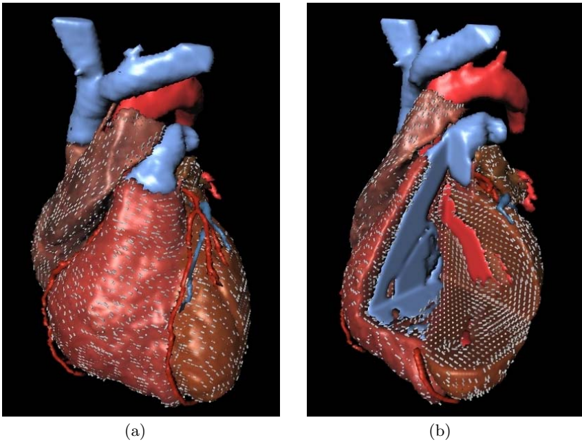
Fig. 6.28. Model of human heart with averaged orientation of myocytes projected on (a) epicardial surface and (b) cutting planes. The orientation was constructed on base of the Visible Man data set, manual editing and interpolation.
