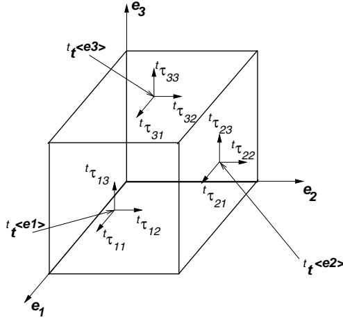
Fig. 4.2. Stresses on faces of cube. The stress vectors {}^t\mathbf{t}^{<\mathbf{e}1>} , {}^t\mathbf{t}^{<\mathbf{e}2>} , and {}^t\mathbf{t}^{<\mathbf{e}3>} are applied to three faces of an infinitesimal cube with the unit normal vectors \mathbf{e}_1 , \mathbf{e}_2 , and \mathbf{e}_3 . The corresponding components of the Cauchy stress tensor {}^t\boldsymbol{\tau} are indicated on the faces.
