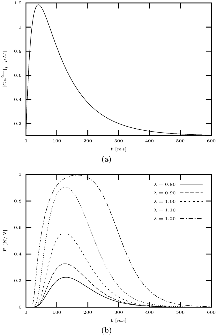
Fig. 8.20. Simulations with 3rd Rice-Winslow-Hunter model by variation of the stretch ratio. (a) An exemplary course of the intracellular calcium concentration [Ca^{2+}]_i is used in the simulations. (b) The development of force F is dependent on the stretch ratio \lambda ranging from 0.8 to 1.2. The force F is normalized with the maximal force F_{max} developable in these simulations.
